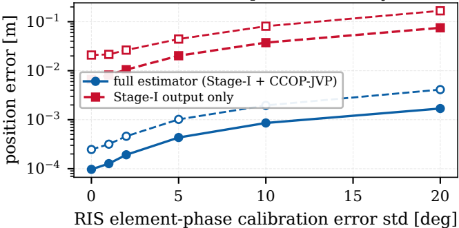
RIS element-phase sensitivity
