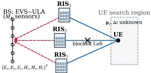
(a) System topology
