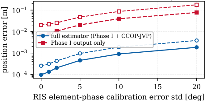
RIS element-phase sensitivity
