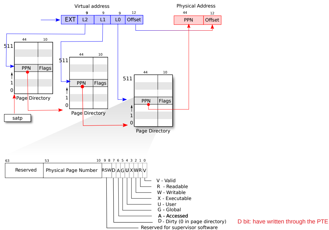
Figure 3.2: RISC-V address translation details.
