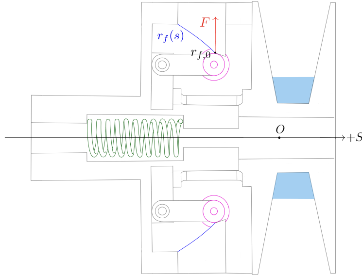
Figure 3.4: Primary clamping mechanism and axial free body of the movable assembly. The flyweight-ramp mechanism closes the primary, while the spring and belt reaction oppose closure.
