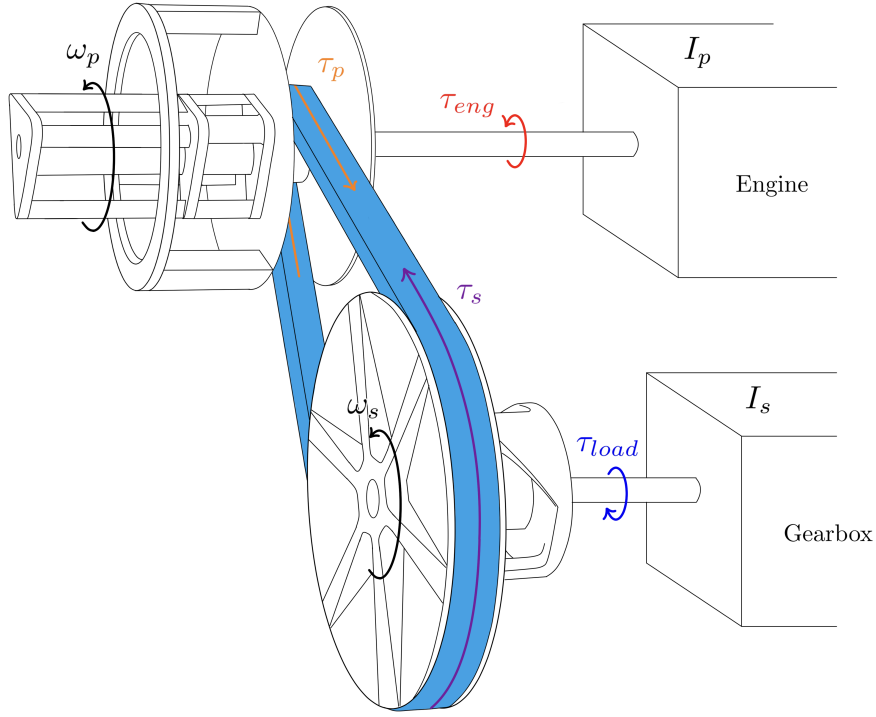
Figure 3.9: Rotating systems and torque path of the engaged CVT. The shaft-side boundaries represent the torque and equivalent inertia presented by the attached systems. The belt remains outside the two pulley-side systems and interacts with them through the contact torques \tau_p and \tau_s . The arrows show the signed directions associated with forward power transfer.
