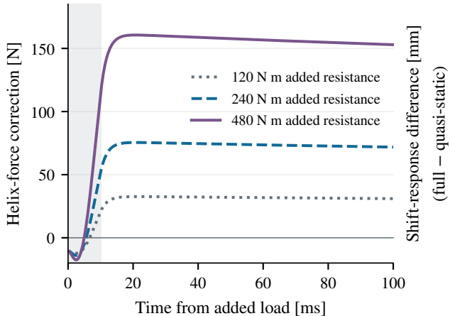
(a) Increasing resisting torque
