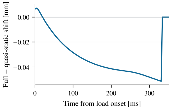
(b) Stock case: resolved separation
