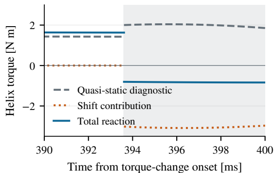
(c) Severe case: algebraic continuation
