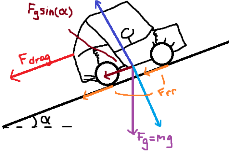
Figure 3.7: Free-body diagram of a vehicle on an incline. The weight mg resolves into mg \sin \alpha along the slope and mg \cos \alpha normal to the surface. Rolling resistance and aerodynamic drag oppose motion.
