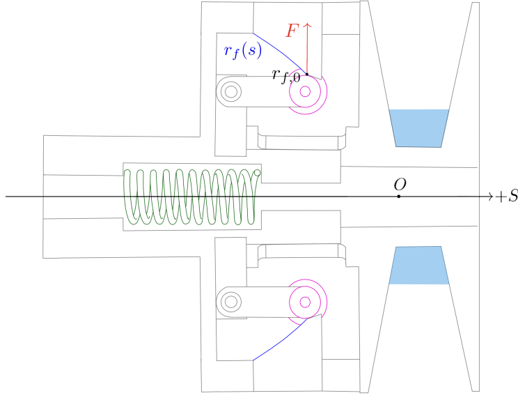
Figure 3.4: Primary clamping mechanism and movable-assembly free body. The flyweight–ramp mechanism applies the axial closing force F_{p,\text{fly}} . The primary spring applies the opposing force F_{p,\text{spring}} , and, after contact, the belt applies the opposing force F_{p,\text{belt}} . The shaded movable sheave and ramp carrier translate together with mass m_p in the positive closing direction +s = +x_p .
