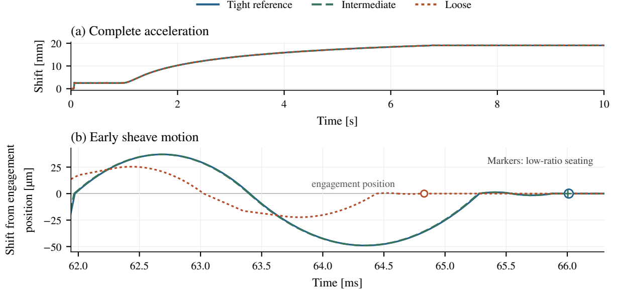
Figure 4.2: Three integrations of the same acceleration. The control triples ( \text{rtol}, \text{atol}, \Delta t_{\text{max}} ) are approximately (1.27 \times 10^{-2}, 1.27 \times 10^{-5}, 25.0 \text{ ms}) for the loose run, (10^{-4}, 10^{-7}, 10 \text{ ms}) for the intermediate run and (10^{-7}, 10^{-10}, 2.5 \text{ ms}) for the tight reference. In (b), negative displacement indicates primary separation. Markers identify low-ratio seating; the reference circle and intermediate cross nearly coincide. Curves retain separate continuous segments. Exact settings and the fixed numerical seating rule are documented in Appendix D.3 .
