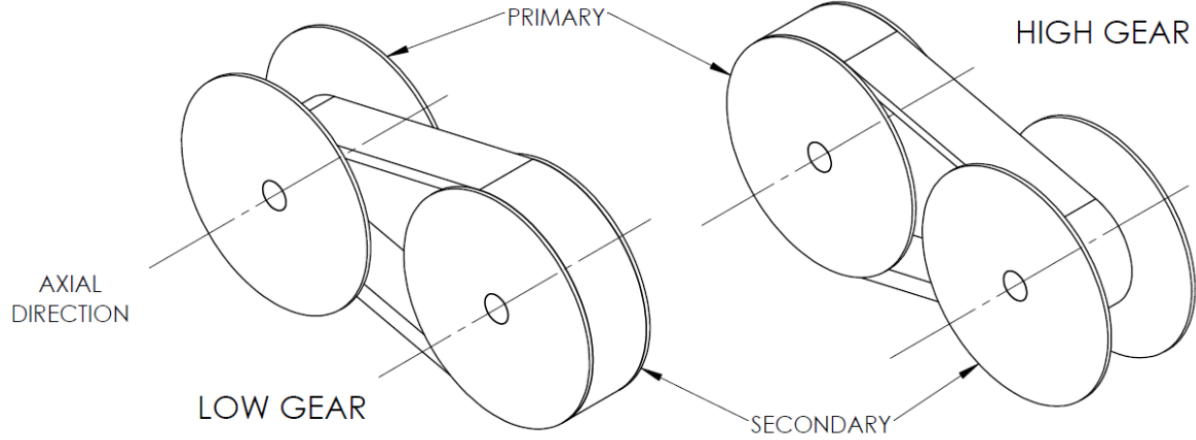
Figure 1.3: Overall layout of the belt-sheave CVT considered in this work. The primary pulley is connected to the engine side, the secondary pulley is connected to the downstream drivetrain, and the rubber V-belt transmits motion and torque between them. (Messick, 2018)
