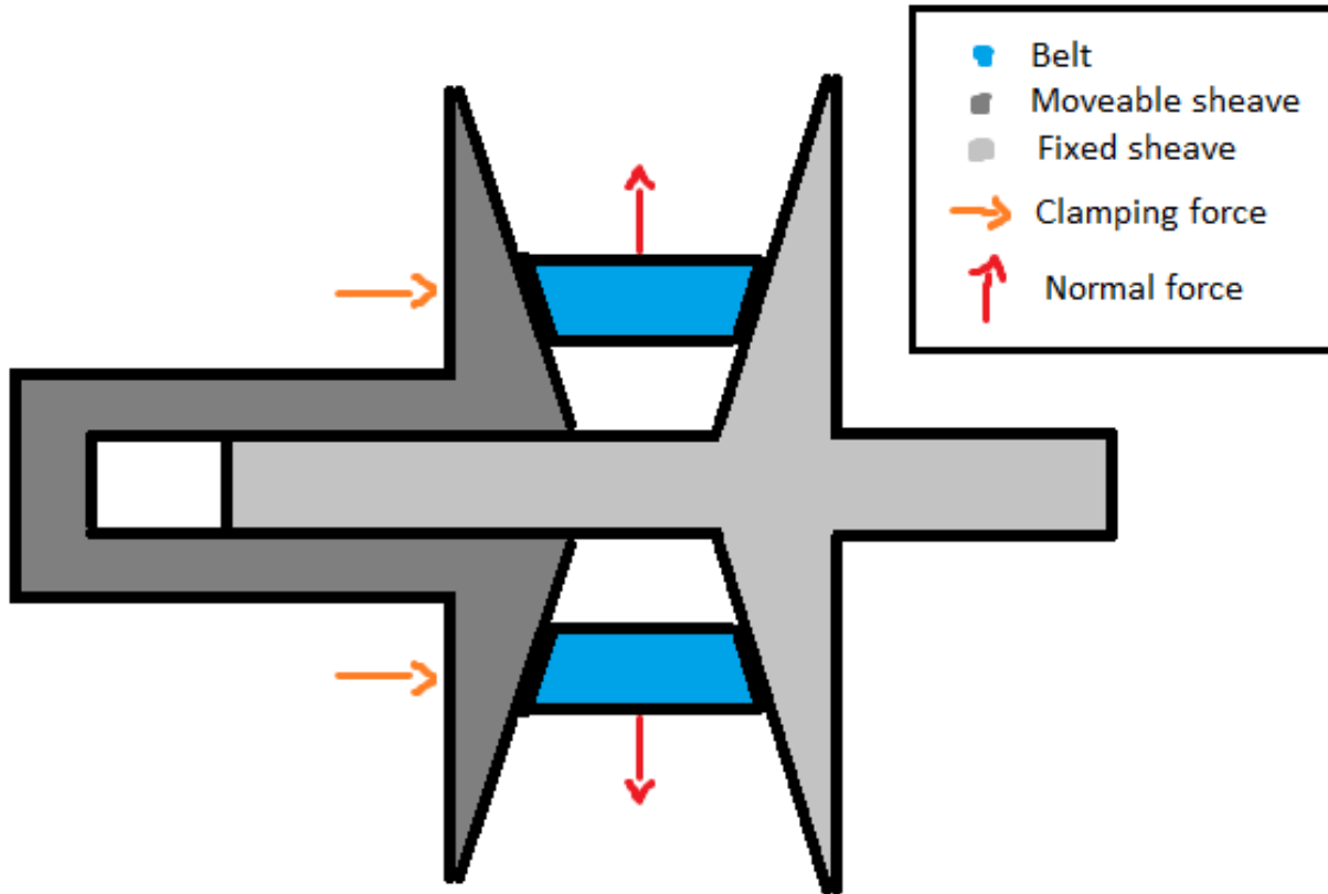
Figure 1.7: Clamping and traction in a rubber V-belt CVT. The belt must be pressed into the sheave faces to generate contact normal force. Frictional traction at this contact allows torque to be transmitted between the pulley and the belt; if the available traction is insufficient, the belt slips.
