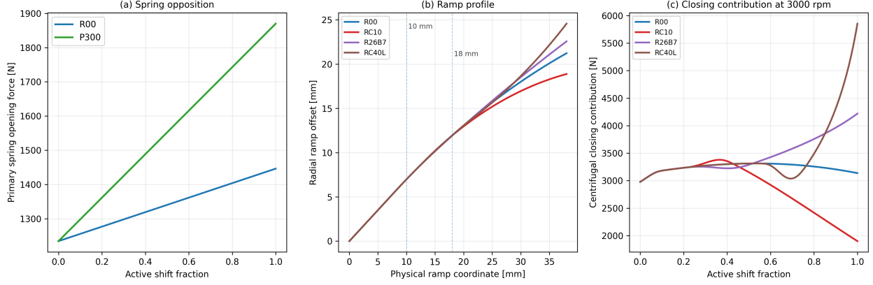
Figure 4.19: Mechanical origin of the selected shift-curve changes. (a) R00 and P300 have the same primary spring force at the selected low-ratio engagement geometry, but the greater P300 stiffness causes the opening force to grow more rapidly with shift. (b) The ramp cases preserve a common early profile and alter the later physical ramp geometry. The dashed positions mark the 10 mm and 18 mm ramp coordinates at which the selected modified families begin to depart from the reference construction. (c) The changed ramp geometry produces different centrifugal closing contributions at the same 3000 rpm primary speed. The ramp changes also alter the retained motion-ratio and flyweight-inertia terms; panel (c) isolates the leading speed-dependent contribution. These maps are mechanism characteristics, while the speed trajectories in Figure 4.18 are obtained only after the complete CVT and vehicle balances are solved.
