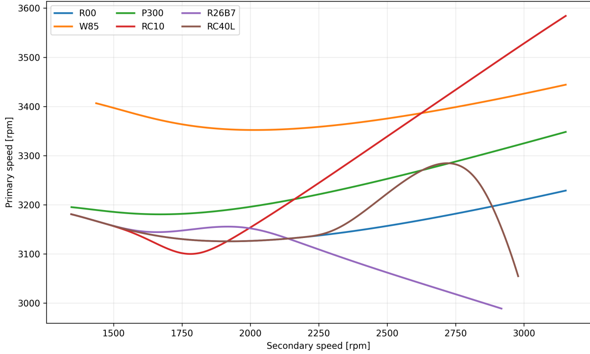
Figure 4.18: Opening-flat free-shift characteristics for selected primary tuning changes. Each curve is the solved primary–secondary speed trajectory while the CVT is engaged, freely shifting, and in stick–stick contact; no speed relation is prescribed. W85 primarily raises the working-speed band, P300 progressively raises primary speed as the shift proceeds, RC10 and R26B7 produce strongly rising and falling characteristics, and RC40L preserves the early response before changing the late-shift shape.
