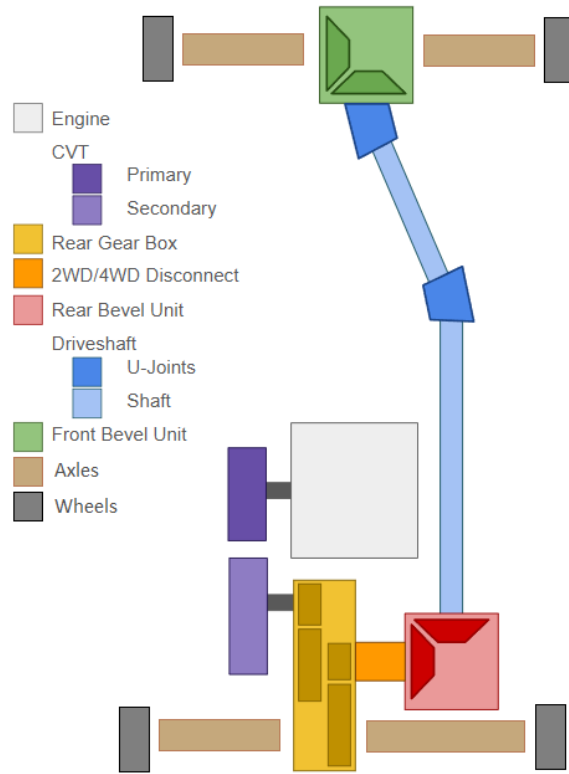
Figure 1.6: Overview of the complete drivetrain architecture considered in this work.
