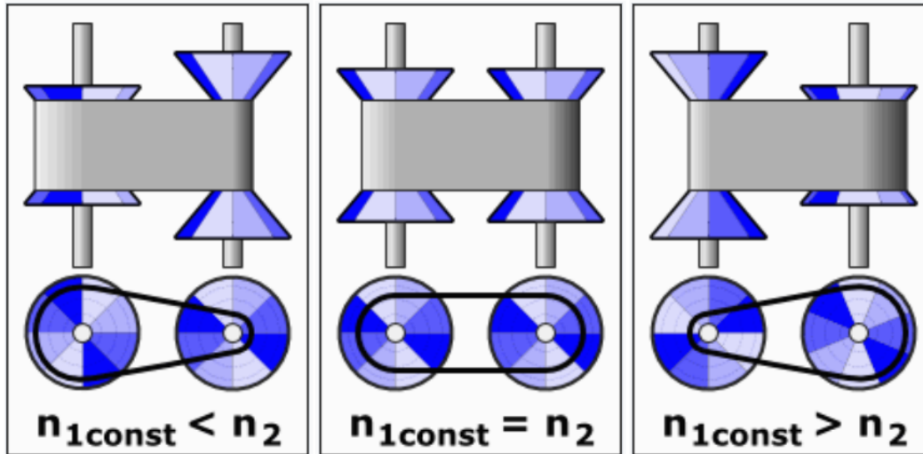
Figure 1.1: Conceptual illustration of a belt-sheave CVT at three different ratios. Changing the axial separation of the conical sheaves alters the effective belt radius, thereby modifying the transmission ratio continuously.
