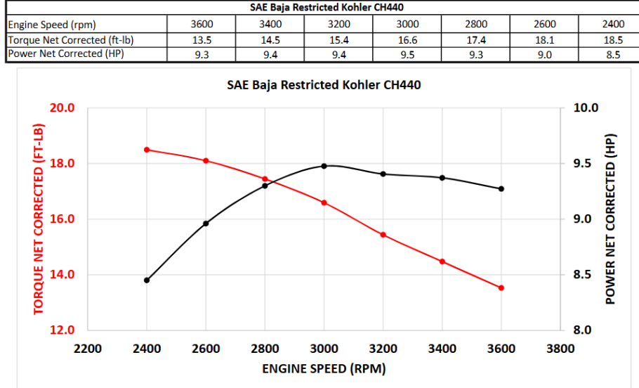
Figure 25: Representative torque and power curves for the Kohler CH440 engine. Torque is supplied as a function of angular velocity and serves as the input mapping in Equation (9.4) .
