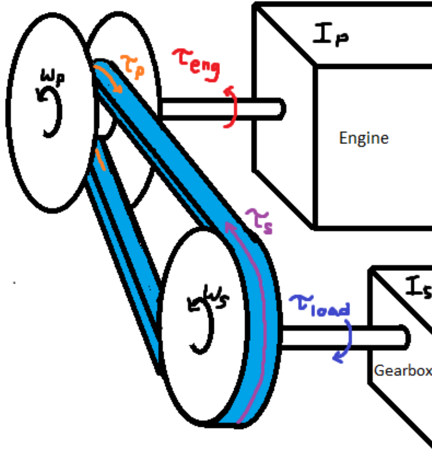
Figure 24: Torque path through the CVT. Engine torque \tau_{\text{eng}} drives the primary pulley with angular speed \omega_p . The primary pulley exchanges torque with the belt, the belt exchanges torque with the secondary pulley, and the secondary pulley drives the downstream drivetrain while opposing the reflected load torque \tau_{\text{load}} .
