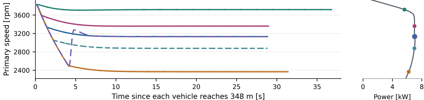
(b) Engine speed during the climb
