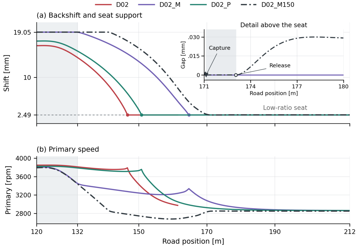
Figure 4.23: Backshift consequences of the three primary-side corrections. (a) Shift position and (b) primary speed, with the entry taper shaded and the common low-ratio seat dashed in (a). D02 ends at sustained primary slip onset. The inset enlarges the gap above the seat for D02_M and D02_M150. Following its initial contact with the stop, D02_M150 remains supported over the shaded inset interval, from about 171.13 m to 173.04 m, approximately 0.51 s, then leaves the seat while both contacts stick. The road remains at 38^\circ throughout the inset. Equal road position retains the different states inherited from the opening flat.
