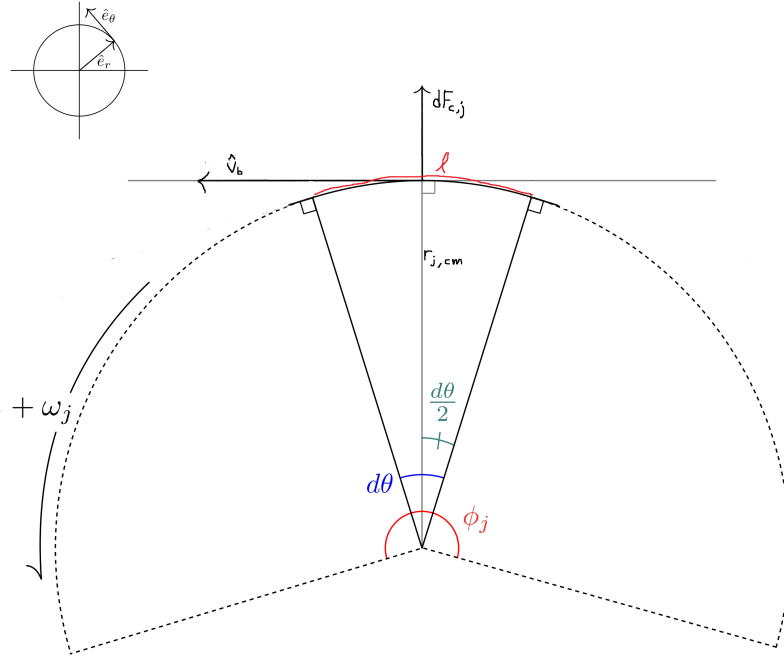
Figure 3.12: Belt wrapped around pulley j . A differential element at angle \theta has arc length d\ell = r_{j,\text{cm}} d\theta and experiences radially outward centrifugal force.
