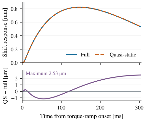
(b) -20 N m over 5 ms, mid travel
