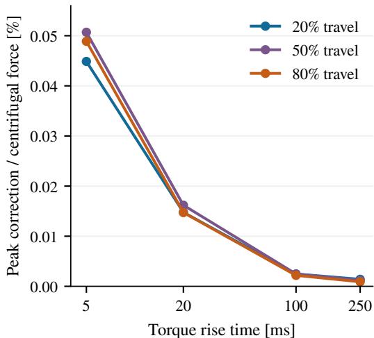
(a) Changing the torque rise time
