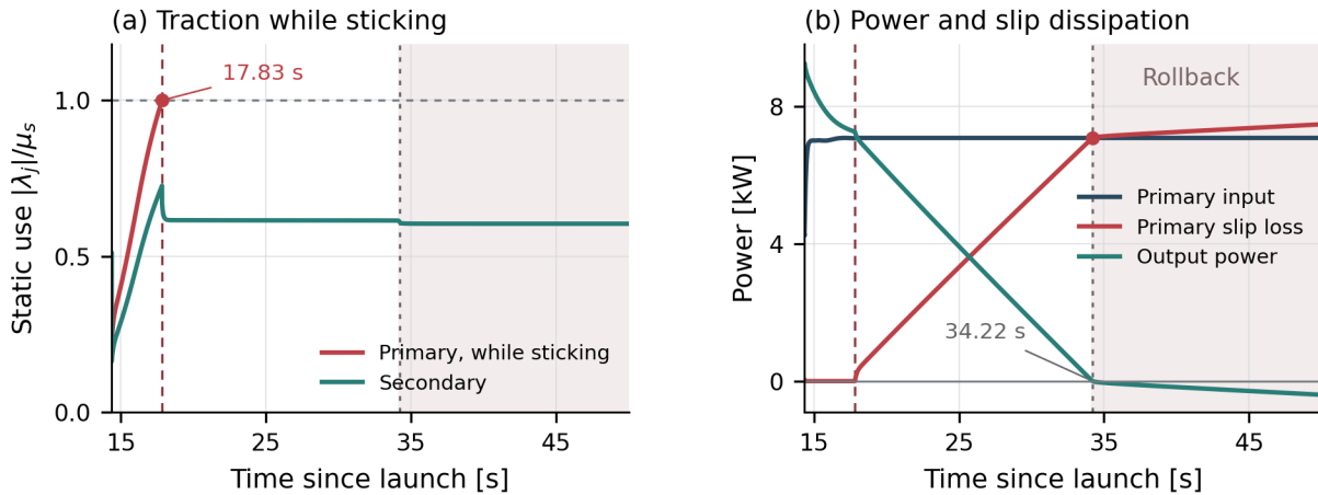
Figure 4.21: D02 from arrival at the low-ratio seat through the retained rollback. (a) Fraction of static traction used while each contact sticks; the primary trace ends when sustained sliding begins. (b) Primary boundary input, primary slip dissipation, and signed output power. Positive output power leaves the CVT; negative output power enters from the vehicle side. Vertical markers identify primary traction loss and the first zero vehicle speed, with rollback shaded. During transients, differences between input, output, and dissipation also include changes in stored mechanical energy.
