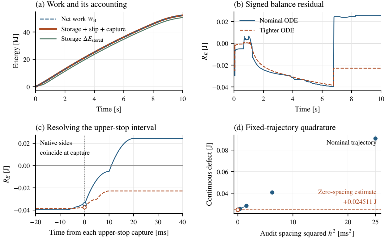
Figure 4.2: Energy accounting for the reference launch. (a) Nominal net work, stored-energy change, and storage plus modeled losses; work and accounted energy overlap at this scale. (b) Signed residuals for the nominal and tighter ODE trajectories, both audited at 0.625 ms maximum spacing. (c) Detail around each trajectory’s upper-stop capture; the incoming and outgoing residuals coincide at the open markers. (d) Continuous-segment defect with the nominal trajectory held fixed. The open point and dashed line mark the two-finest-grid, second-order zero-spacing estimate. Native event sides are retained; lines and work quadrature do not bridge velocity resets.
