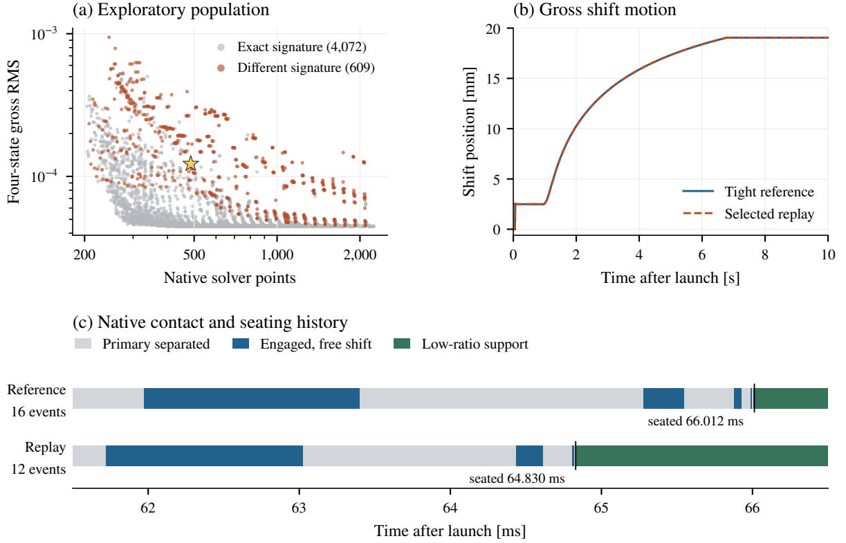
Figure 4.4: Gross motion and contact history. (a) All 4,681 completed exploratory runs, grouped by exact signature agreement, not transition count; the 264 failed runs have no trajectory norm. Native solver points are a work proxy, not function evaluations. The star selects the median different-signature setting. (b) Its replay and the tight reference have nearly coincident ten-second shift curves. (c) Their native absolute-time histories differ during engagement and seating. The shortest intervals cannot be resolved at this scale; their durations are retained in Table D.12 . Traces are not joined across resets.
