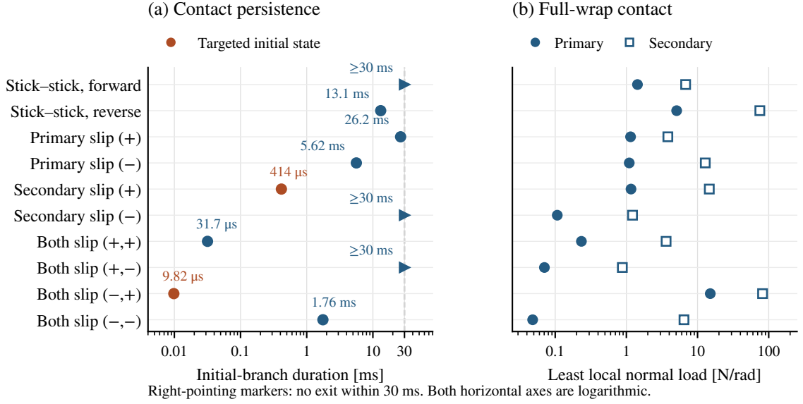
Figure 4.1: Persistence and local contact loading for ten canonical initial contact states. (a) Time to first transition; orange marks the supplied initial-state anchors. (b) Least normal loading per unit wrap angle on each pulley over engaged states in the 30 ms continuation. Minima may follow a contact change and need not coincide between pulleys. Deadzone intervals are excluded because they have no engaged full-wrap field.
