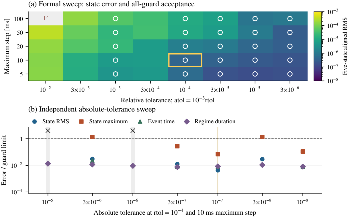
Figure 4.3: Formal numerical refinement. (a) Each cell is one of the 40 tested tolerance/maximum-step combinations. Colour shows the five-state aligned RMS; circles additionally require every state, timing and history guard to pass; F marks the failed integration. (b) Each error is divided by its own guard limit, so values above one fail. Crosses identify different signatures, for which aligned state and corresponding event-time errors are undefined. Regime-duration error remains defined. Gold marks the research setting. No boundary is inferred between sampled settings; maximum step is a cap on adaptive integration.
