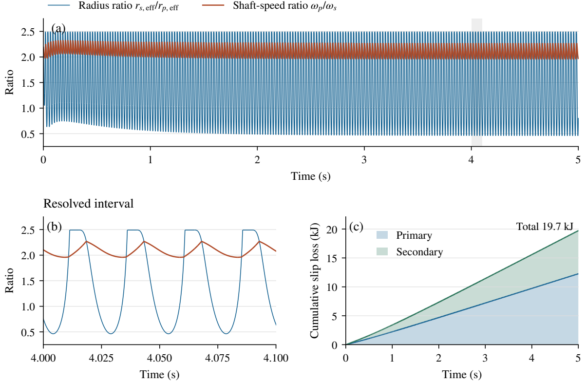
Figure 4.7: Internal response under reconstructed feedback. (a) Shaft-speed and effective-radius ratios over the complete run. The shaded interval is expanded in (b), showing the actual motion rather than an averaged ratio. (c) Stacked cumulative slip losses at the primary and secondary contacts; the upper boundary is their sum. Continuous segments retain their separate event endpoints.
