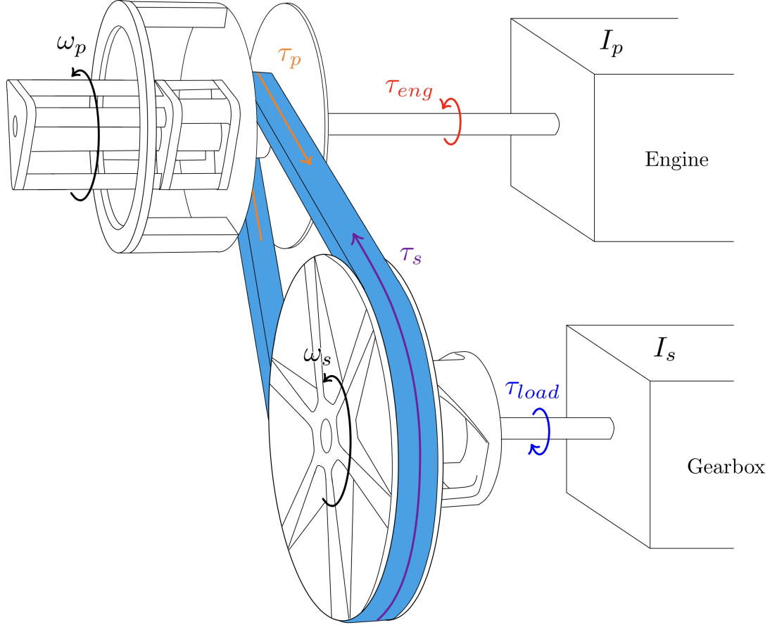
Figure 3.11: Torque path through the CVT. Engine torque \tau_{eng} drives the primary pulley with angular speed \omega_p . The primary pulley exchanges torque with the belt, the belt exchanges torque with the secondary pulley, and the secondary pulley drives the downstream drivetrain while opposing the reflected load torque \tau_{load} .
