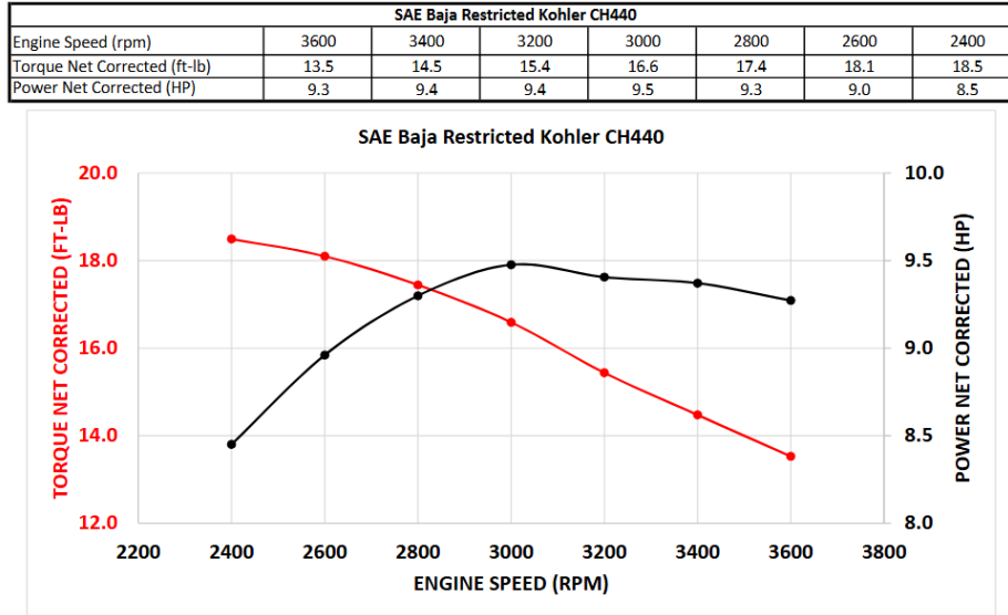
Figure 3.12: Representative torque and power curves for the Kohler CH440 engine. Torque is supplied as a function of angular velocity and serves as the input mapping in Equation (3.5.1).
