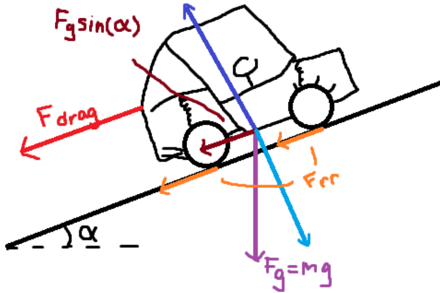
Figure 3.13: Free-body diagram of a vehicle on an incline. The weight mg resolves into mg \sin \alpha along the slope and mg \cos \alpha normal to the surface. Rolling resistance and aerodynamic drag oppose motion.
