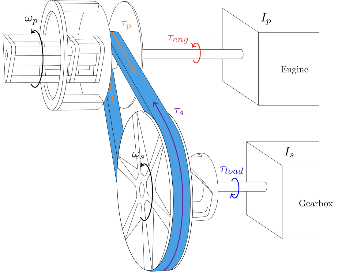
Figure 24: Torque path through the CVT. Engine torque \tau_{\text{eng}} drives the primary pulley with angular speed \omega_p . The primary pulley exchanges torque with the belt, the belt exchanges torque with the secondary pulley, and the secondary pulley drives the downstream drivetrain while opposing the reflected load torque \tau_{\text{load}} .
