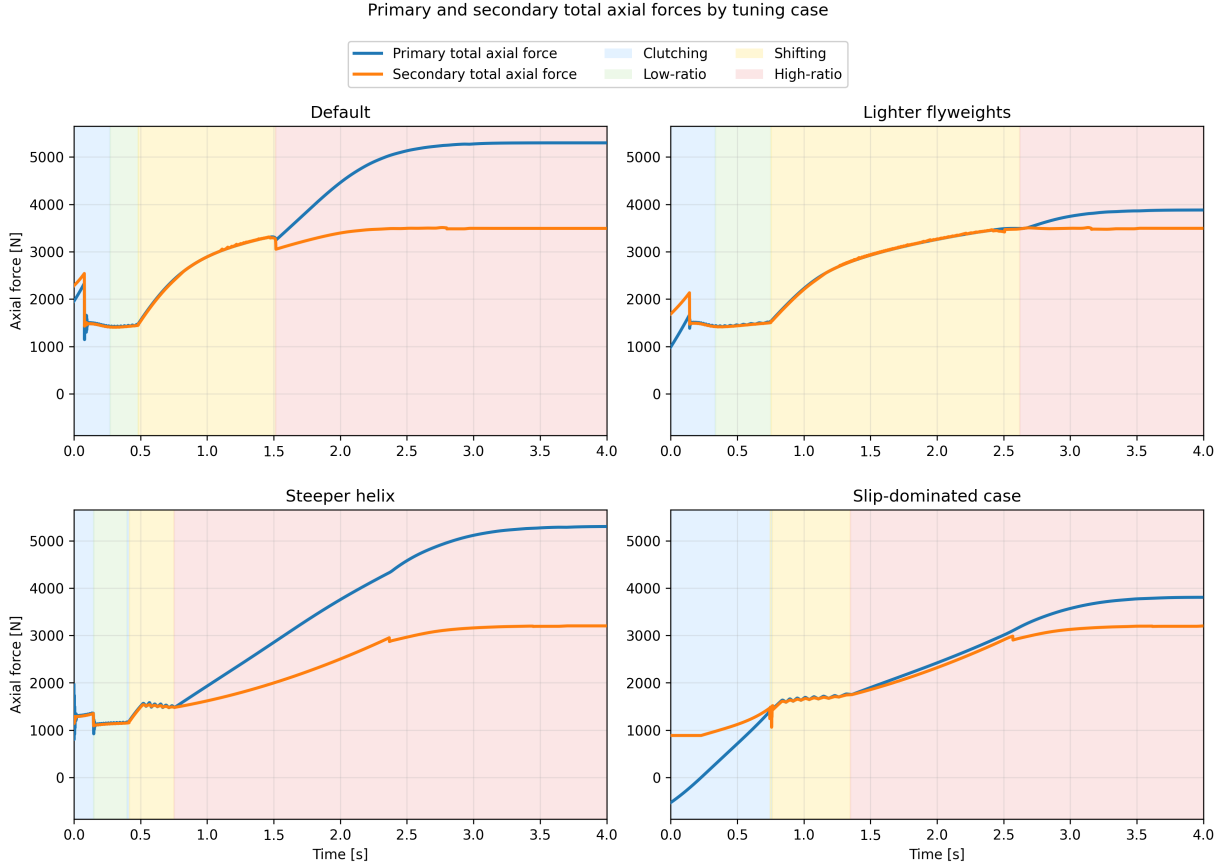
Figure 30: Primary and secondary total axial forces during launch for the four tuning cases. Blue curves show total primary axial force, orange curves show total secondary axial force. Background shading indicates the clutching, low-ratio, shifting, and high-ratio phases defined earlier.
