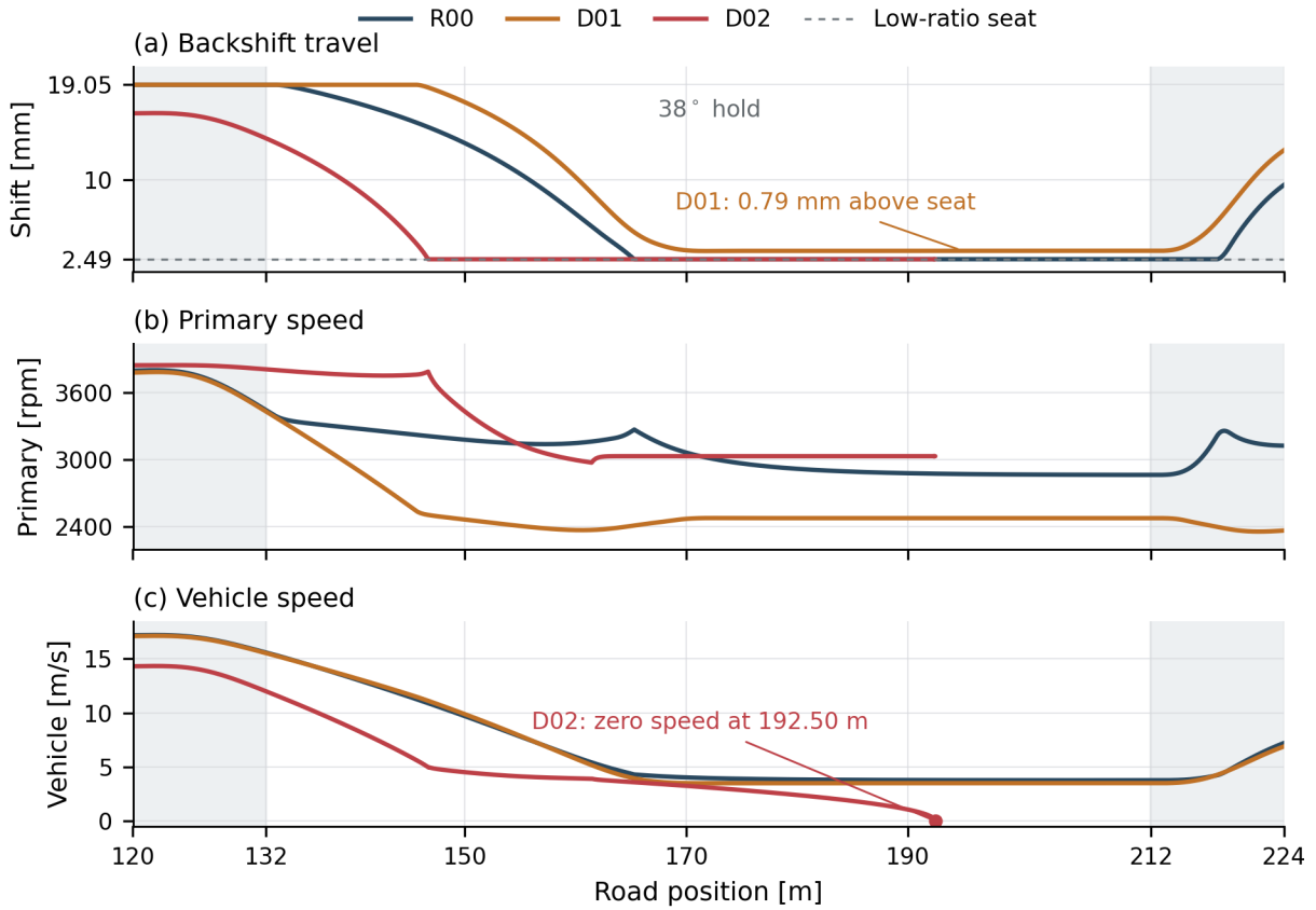
Figure 4.17: Response to the first severe climb. The shaded bands mark the entry and exit tapers; the intervening road holds 38^\circ . The dashed line in (a) marks the low-ratio seat. All three D02 traces end at its first zero vehicle speed, near 192.50 m. Equal road position means equal imposed grade, not equal elapsed time or inherited state.
