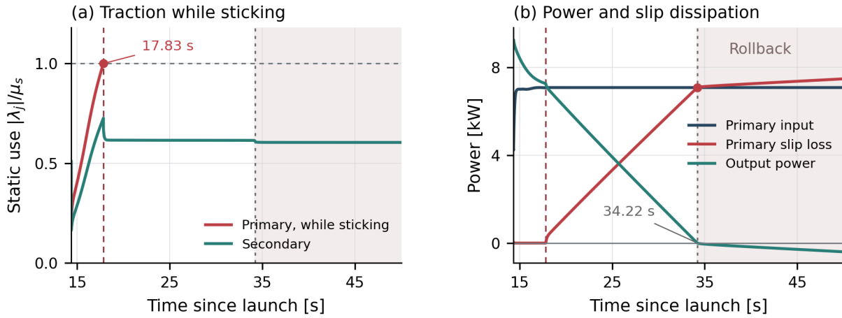
Figure 4.18: D02 from arrival at the low-ratio seat through the retained rollback. (a) Fraction of static traction used while each contact sticks; the primary trace ends when sustained sliding begins. (b) Primary boundary input, primary slip dissipation, and signed output power. Positive output power leaves the CVT; negative output power enters from the vehicle side. Vertical markers identify primary traction loss and the first zero vehicle speed, with rollback shaded. During transients, differences between input, output, and dissipation also include changes in stored mechanical energy.
