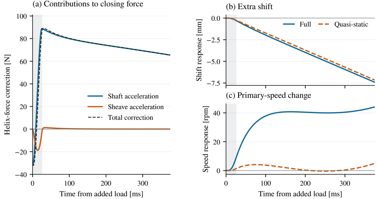
Figure 4.11: Response with the nominal estimated secondary to an added torque of -120 \text{ N m} over 25 ms, with the ramp shaded. (a) Signed helix-force corrections evaluated on the full model’s motion. (b,c) Each model’s loaded motion minus its own unforced continuation. Both contacts stick and the sheaves remain free to shift throughout all four continuations. The force correction and the independently integrated response are different comparisons.
