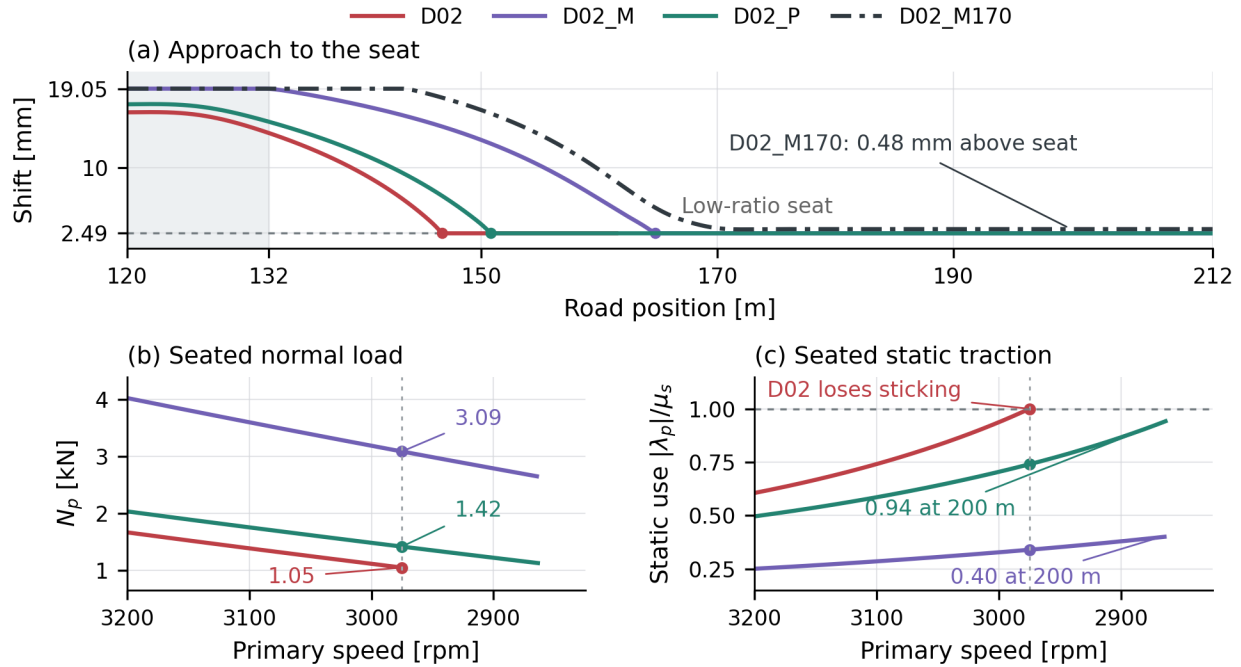
Figure 4.21: Clamping and backshift under the three primary-side corrections. (a) Approach to the common low-ratio seat, with the hill-entry taper shaded. Equal road position retains the different states inherited from the opening flat. (b) Total primary normal load and (c) static utilization during seated sticking on the 38^\circ hold, after the seating transitions. Markers in (b,c) identify the comparison near 2975 rpm; the repair utilization annotations refer to states near 200 m. D02 traces end at sustained primary slip onset. D02_M170 is absent from (b,c) because it does not reach the seat on the constant 38^\circ climb.
