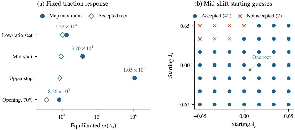
Figure 4.4: Fixed-traction conditioning and sticking-search outcomes. (a) Unmasked maxima over four 241 \times 241 static-capacity maps, contrasted with values at the accepted roots. All use the same row/column-equilibrated eight-variable matrix of Equation (B.2.3) . Opening denotes the constructed state at 70% engaged travel and -20 mm/s. (b) All 7 \times 7 mid-shift starting guesses: 42 are accepted and seven are not. The star marks the common accepted root, not a starting guess or an iteration path. Neither panel establishes global uniqueness.
