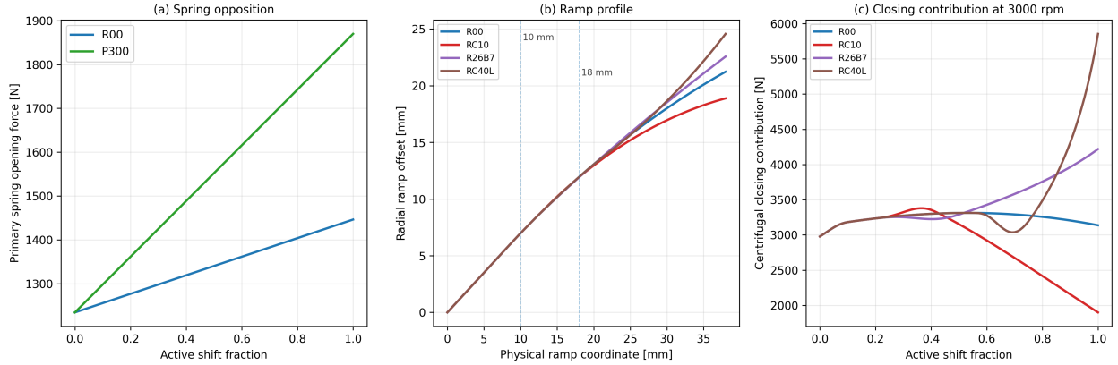
Figure 4.18: Mechanical origin of the selected shift-curve changes. (a) Primary spring opening force for R00 and P300, matched at the low-ratio engagement geometry. (b) Physical ramp profiles: RC10 and R26B7 preserve the first 10 mm of the reference ramp, while RC40L preserves the first 18 mm; these distances are ramp coordinates rather than movable-sheave travel. (c) Leading centrifugal closing contribution at the same 3000 rpm primary speed. The complete actuator also retains the corresponding motion-ratio and flyweight-inertia terms, so panel (c) isolates one contribution rather than replacing the full dynamic force law. In (a) and (c), active shift fraction runs from zero at the low-ratio seat to one at the upper primary stop.
