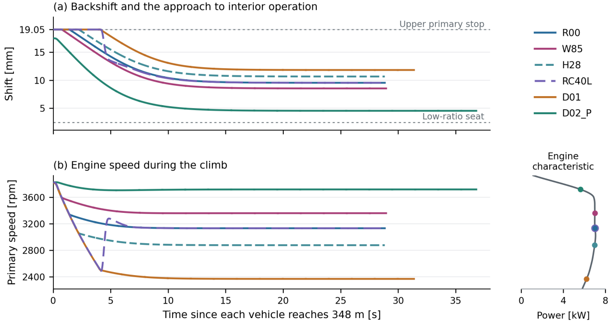
Figure 4.23: Approach to sustained climbing on the 18^\circ hill. (a) Shift position, with the common upper primary stop and low-ratio seat marked. (b) Primary speed. The engine-power curve on the right shares its speed scale, with coloured markers at the late mean primary speeds. Time is measured from each vehicle's arrival at 348 m; each trace ends at 596 m, before the grade decreases. Equal elapsed time does not imply equal road position. The later R00 and RC40L traces nearly coincide in both panels; their power-curve markers also overlap.
