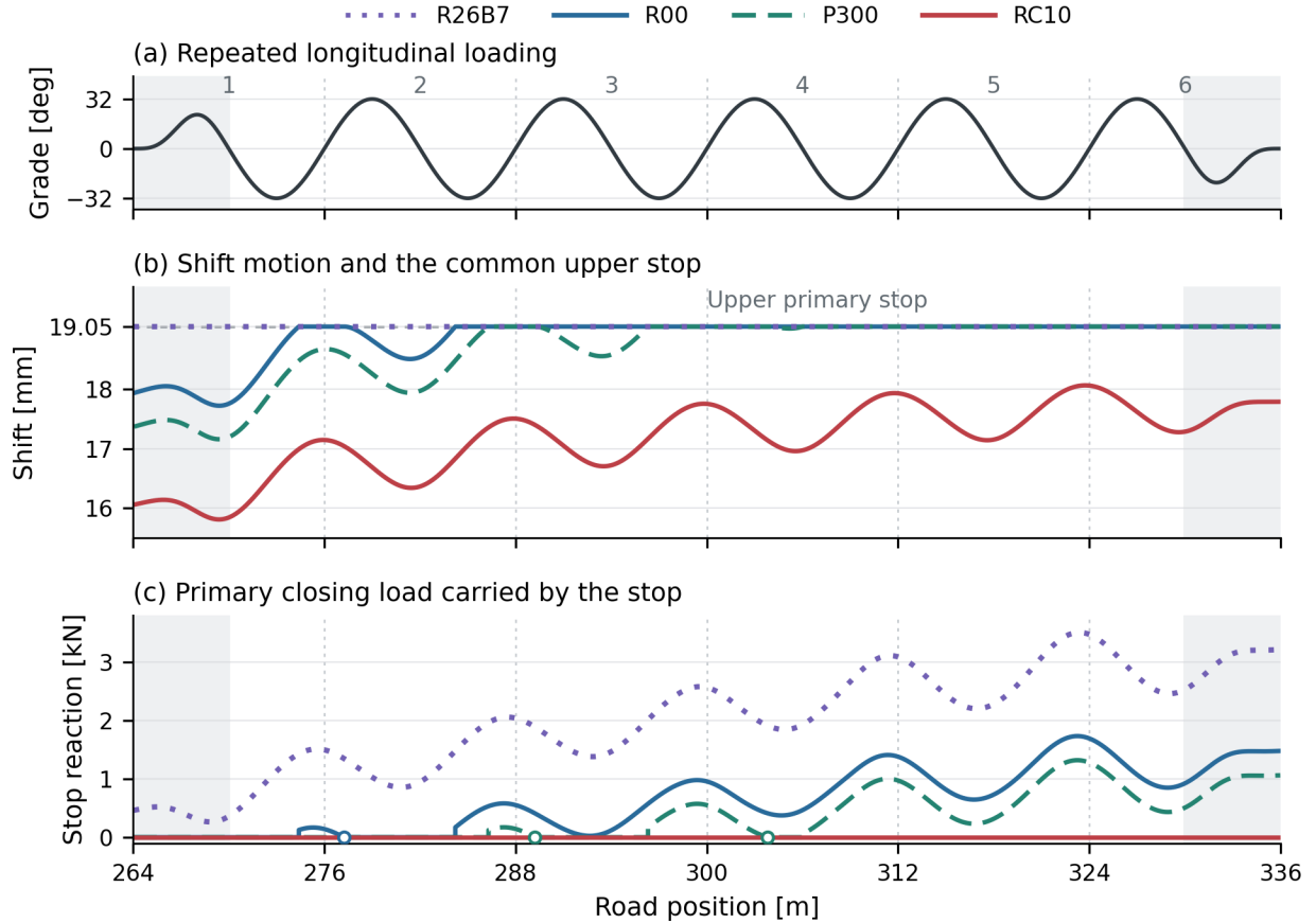
Figure 4.22: Repeated loading from 264 m to 336 m. (a) Road grade, with cycles numbered and the 6 m end tapers shaded; cycles 2–5 have the full \pm 32^\circ amplitude throughout. (b) Shift position; supported traces coincide at the common upper stop. (c) Primary stop reaction, zero while the primary is away from the stop. Open circles mark recorded releases from support. Equal road position aligns the imposed grade, not elapsed time or the states inherited from the preceding road.
