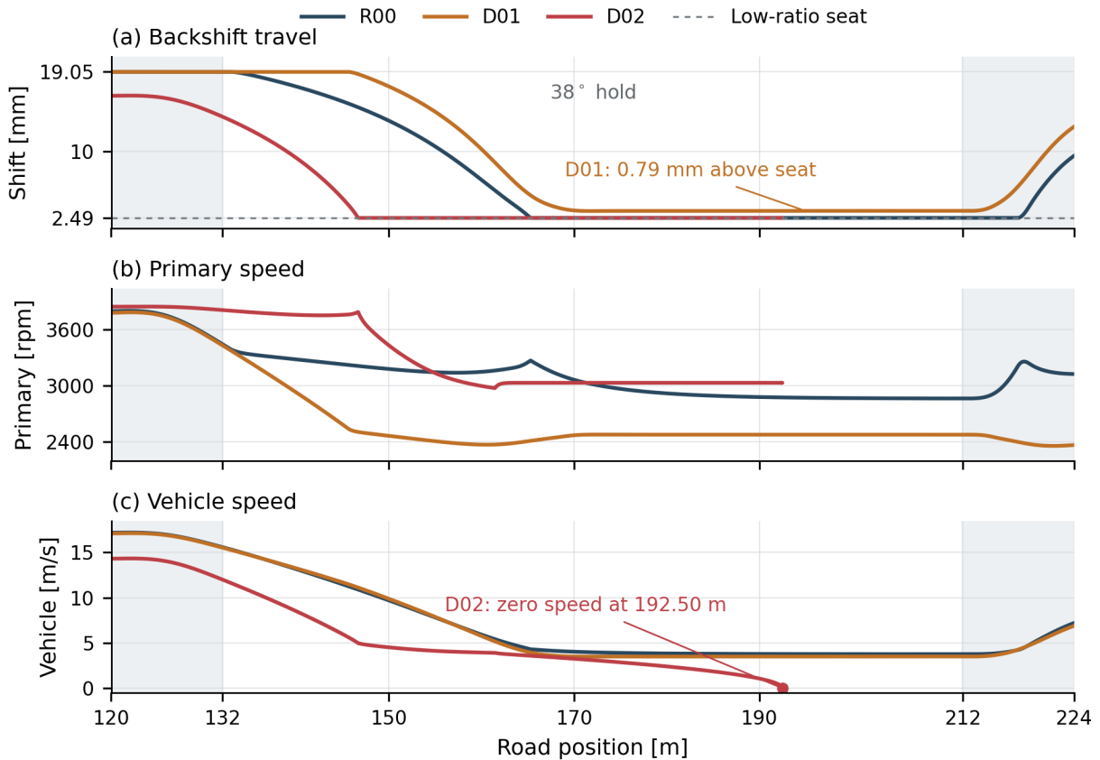
Figure 4.19: Response to the first severe climb. The shaded bands mark the entry and exit tapers; the intervening road holds 38°. The dashed line in (a) marks the low-ratio seat. All three D02 traces end at its first zero vehicle speed, near 192.50 m. Equal road position means equal imposed grade, not equal elapsed time or inherited state.
