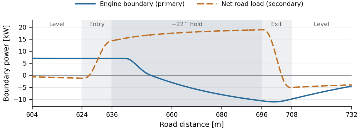
Figure 4.24: R00 boundary powers during the final descent. The primary trace is \tau_{B,p}\omega_p ; the secondary trace is \tau_{B,s}\omega_s , equal to the net road force times vehicle speed. Grey shading marks the descent, with darker shading for the constant -22^\circ grade. Negative primary power denotes absorption by the engine boundary. These powers need not balance while the vehicle and transmission gain or lose kinetic energy.
