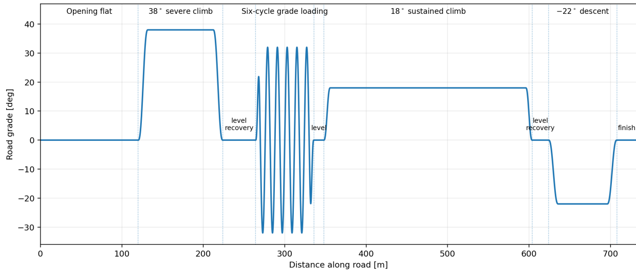
Figure 4.16: Distance-indexed road grade used by every configuration on the common 732 m course. The first 120 m are level. A smooth 12 m entry leads to an 80 m hold at 38^\circ , followed by a 12 m exit and 40 m of level recovery. From 264 m to 336 m, the road completes six 12 m grade cycles with a peak amplitude of \pm 32^\circ , followed by 12 m of level road. The second climb uses an 8 m entry, a 240 m hold at 18^\circ , and an 8 m exit, followed by 20 m of level recovery. The final load change is a -22^\circ descent with 12 m entry and exit transitions around a 60 m constant-grade section, followed by a 24 m level finish. The cyclic region changes only the longitudinal road grade; suspension motion, wheel unloading, tire normal-load variation, and airborne vehicle dynamics are not represented.
