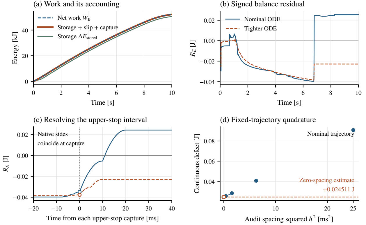
Figure 4.1: Energy accounting for the reference launch. (a) Nominal net work, stored-energy change, and storage plus modeled losses; work and accounted energy overlap at this scale. (b) Signed residuals for the nominal and tighter ODE trajectories, both audited at 0.625 ms maximum spacing. (c) Detail around each trajectory’s upper-stop capture; the incoming and outgoing residuals coincide at the open markers. (d) Continuous-segment defect with the nominal trajectory held fixed. The open point and dashed line mark the two-finest-grid, second-order zero-spacing estimate. Native event sides are retained; lines and work quadrature do not bridge velocity resets.
