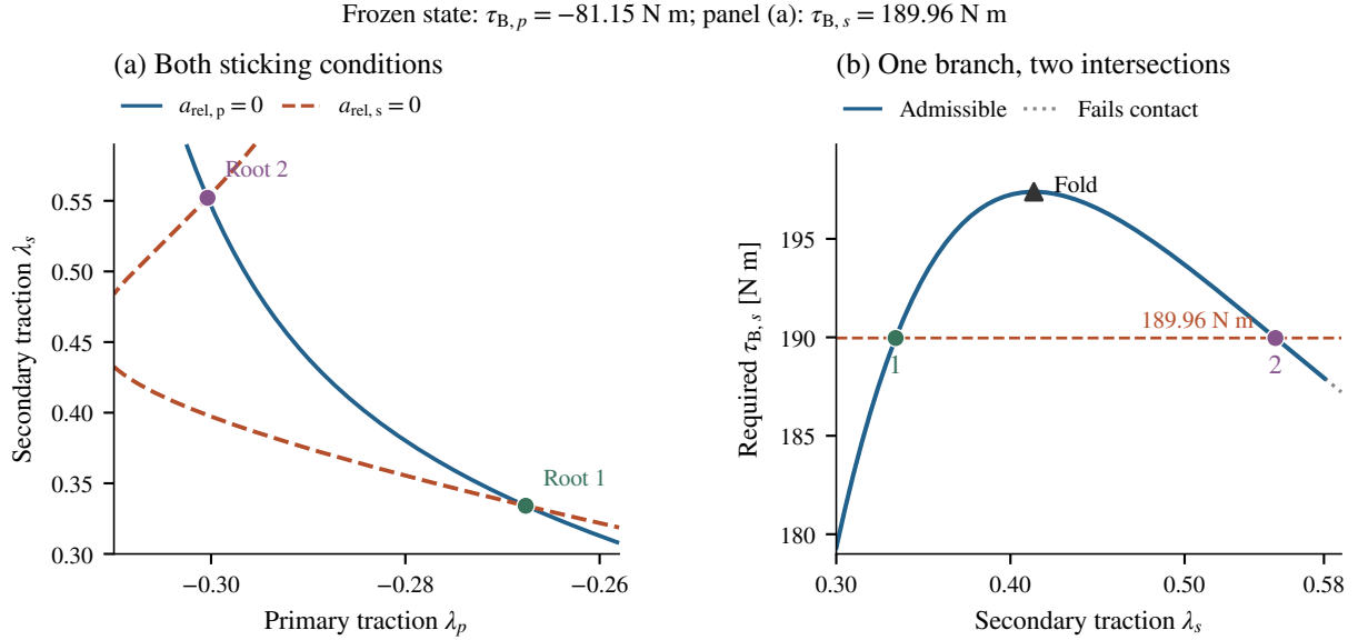
Figure 4.5: Two sticking roots at one frozen state: 95% engaged travel, -40 mm/s opening speed and 3000 rpm primary speed. (a) Both acceleration residuals vanish at each marked intersection under the displayed shaft-boundary torques. (b) The required secondary boundary torque along the same locally corrected sticking branch, with primary boundary torque fixed. The horizontal line intersects it at the same two roots. Secondary traction is a branch coordinate, not time or shift position. The dotted continuation beyond loss of local wrap compression is mathematical only. Exact inputs and signed responses are given in Section D.4.
