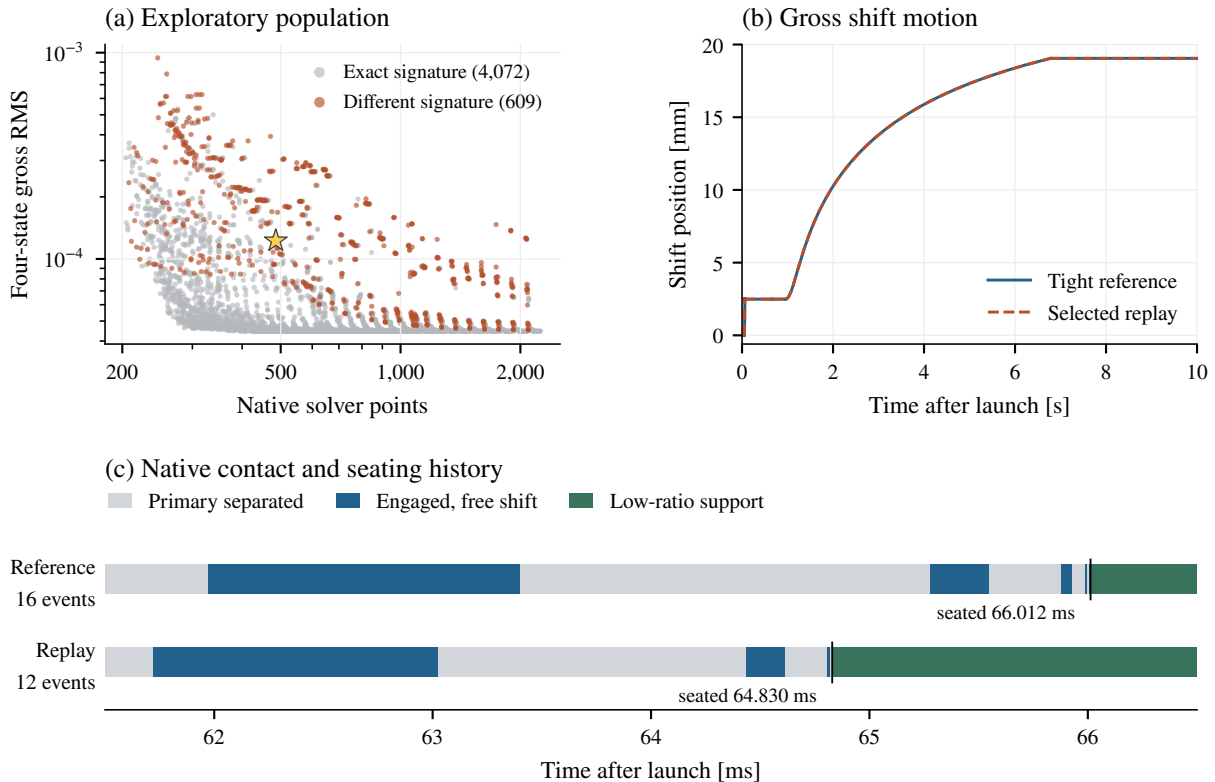
Figure 4.3: Gross motion and contact history. (a) All 4,681 completed exploratory runs, grouped by exact signature agreement, not transition count; the 264 failed runs have no trajectory norm. Native solver points are a work proxy, not function evaluations. The star selects the median different-signature setting. (b) Its replay and the tight reference have nearly coincident ten-second shift curves. (c) Their native absolute-time histories differ during engagement and seating. The shortest intervals cannot be resolved at this scale; their durations are retained in Table D.12. Traces are not joined across resets.
