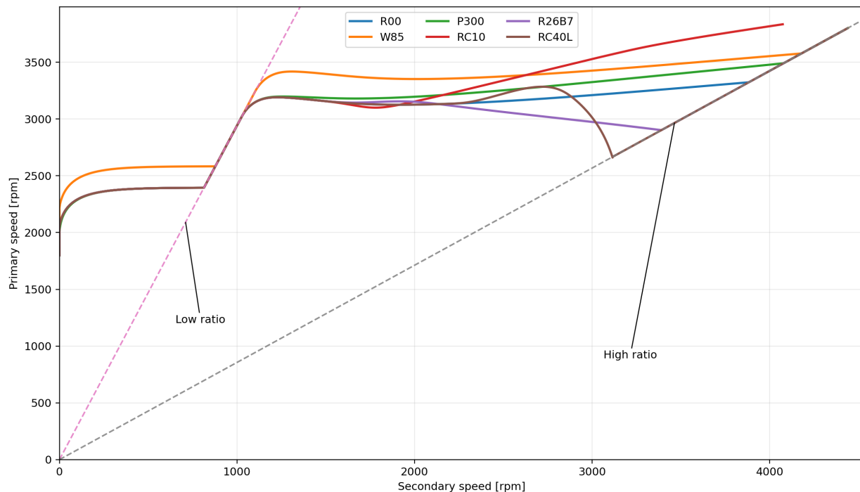
Figure 4.17: Complete opening-flat shift curves for the six selected primary hardware configurations, from the initial state through the last recorded point before 120 m. The solid curves retain the initial disengaged motion, launch slip, supported motion, and free shift. The dashed lines are the no-slip speed relations at the geometric low- and high-ratio limits.
