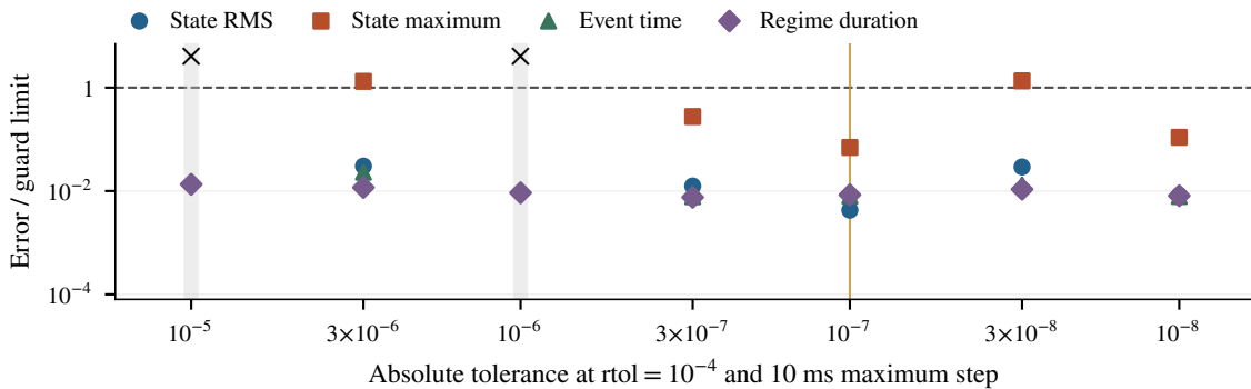
(b) Independent absolute-tolerance sweep
