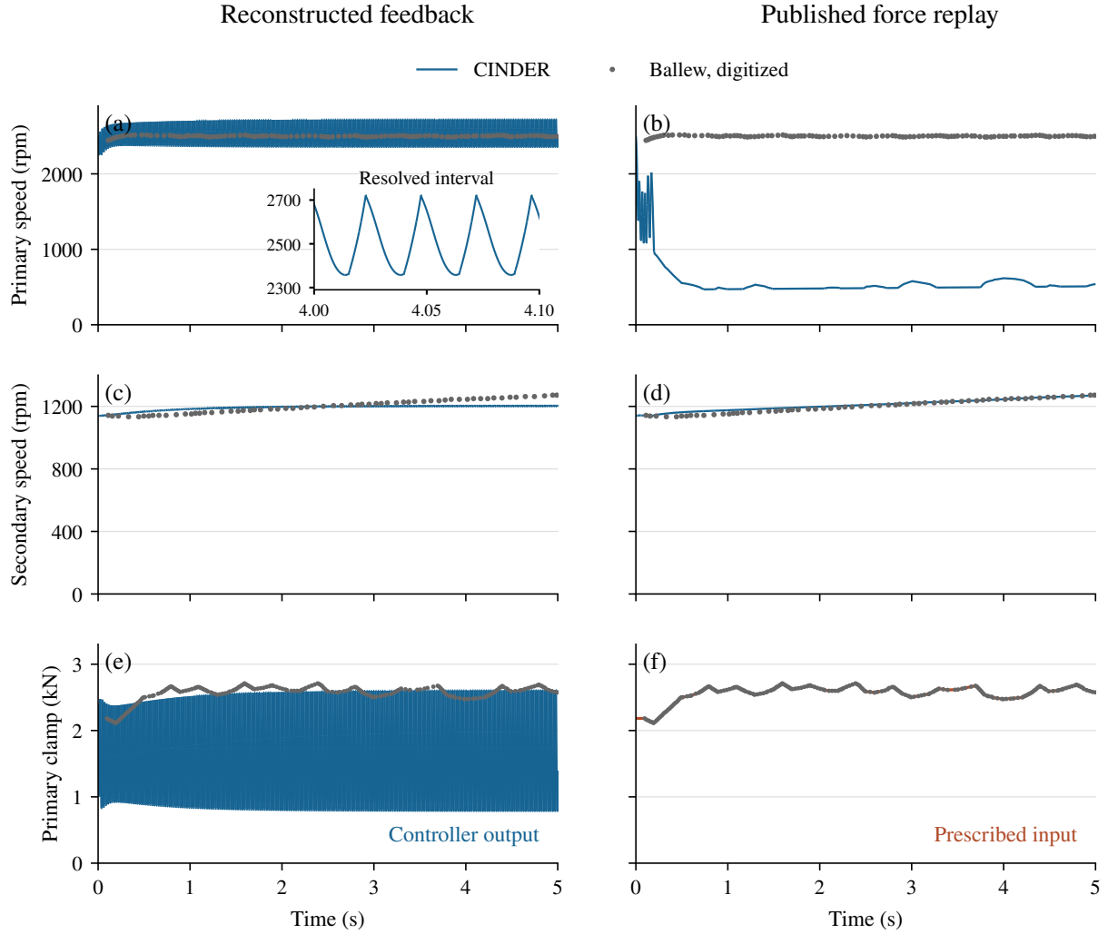
Figure 4.6: Reconstructed feedback and prescribed-force replay against Ballew’s simulated histories. Corresponding panels use the same scales. Points are digitized from Figures 41 and 45 (?); the CINDER traces are unsmoothed, and the inset resolves the primary-speed oscillation over 0.1 s. The primary force is a controller output in (e) and a prescribed input in (f). Both protocols share the secondary clamp and shaft boundaries.
