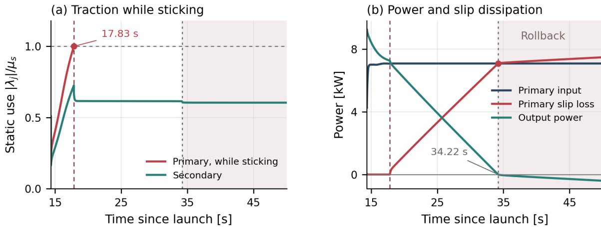
Figure 4.20: D02 from arrival at the low-ratio seat through the retained rollback. (a) Fraction of static traction used while each contact sticks; the primary trace ends when sustained sliding begins. (b) Primary boundary input, primary slip dissipation, and signed output power. Positive output power leaves the CVT; negative output power enters from the vehicle side. Vertical markers identify primary traction loss and the first zero vehicle speed, with rollback shaded. During transients, differences between input, output, and dissipation also include changes in stored mechanical energy.
