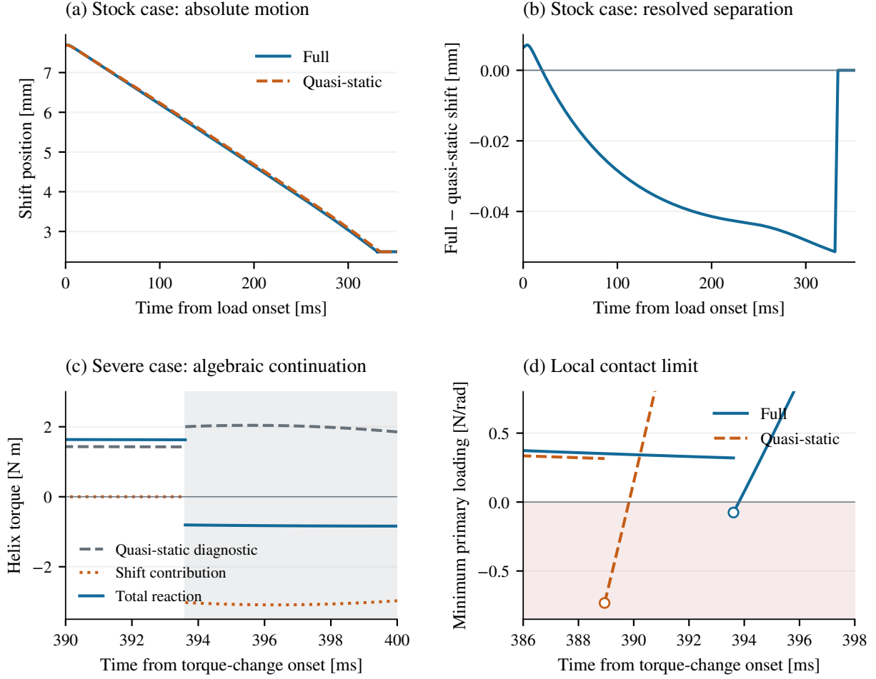
Figure D.3: Supporting comparisons and the reversal limit. (a,b) Stock-case motion and its small, resolved shift separation. (c) The full reversal’s signed reaction, with the region after the local-contact failure shaded. The quasi-static diagnostic is evaluated on the full trajectory; it is not the separately integrated reduced model. (d) Local primary-wrap minima for the two formal continuations. Hollow points denote the exact outgoing states; the region below zero requires tensile contact. Curves on different event sides are not joined. The post-event traces in (c,d) diagnose the failed contact assumption and are not admissible continuations.
