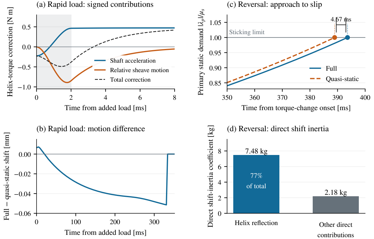
Figure 4.10: Reference-secondary transients. (a,b) Added secondary torque of -120 N m over 2 ms, with 300^\circ preload: signed torque corrections on the full trajectory and independently integrated shift difference. Shading marks the ramp. (c,d) Primary torque reduced to -28 N m over 50 ms, with 270^\circ preload: traction demand and the direct shift-inertia budget. Curves in (c) end at their incoming traction-limit states; (d) uses the full model's incoming state. The outgoing states fail local belt contact. Time is measured from each torque-change onset.
