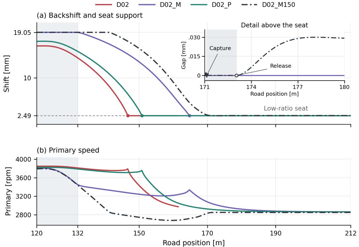
Figure 4.23: Backshift consequences of the three primary-side corrections. (a) Shift position and (b) primary speed, with the entry taper shaded and the common low-ratio seat dashed in (a). D02 ends at sustained primary slip onset. The inset enlarges the gap above the seat for D02_M and D02_M150. Following its initial contact with the stop, D02_M150 remains supported over the shaded inset interval, from about 171.13 m to 173.04 m, approximately 0.51 s, then leaves the seat while both contacts stick. The road remains at 38^\circ throughout the inset. Equal road position retains the different states inherited from the opening flat.
