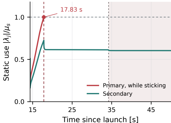
(a) Traction while sticking
