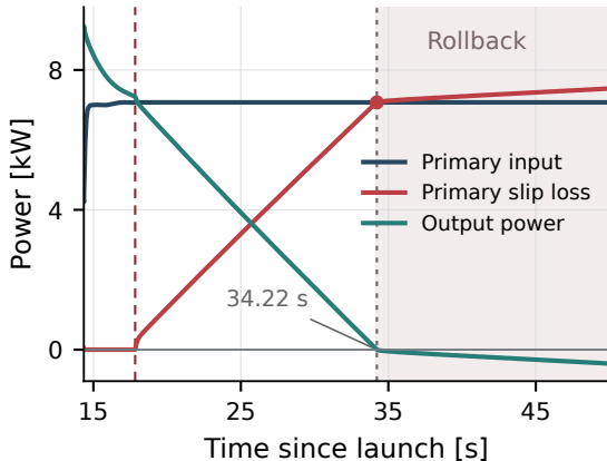
(b) Power and slip dissipation
