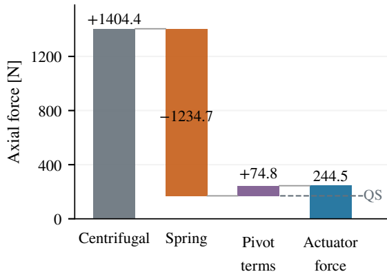
(b) Force just after engagement
