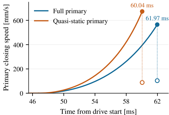
(a) Approach and first engagement
