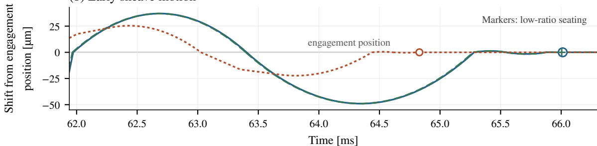
(b) Early sheave motion
