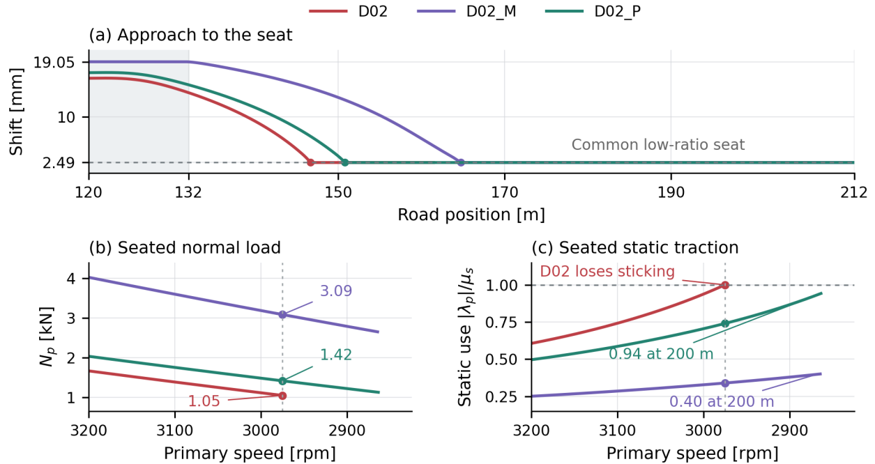
Figure 4.22: Severe-hill repair comparison. (a) Shift paths, with the entry taper shaded and the low-ratio seat dashed. (b,c) Total primary normal load and static utilization during seated sticking on the 38^\circ hold, after the seating transitions. Markers identify the comparison near 2975 rpm. D02 ends at sustained primary slip onset; repair annotations refer to states near 200 m.
