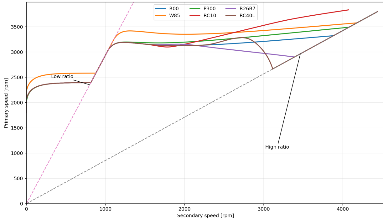
Figure 4.18: Opening-flat free-shift characteristics for selected primary hardware changes. Each solid curve is the solved primary–secondary speed trajectory while the CVT is engaged, freely shifting, and in stick–stick contact. The dashed lines show the fixed no-slip speed relations at the geometric low-ratio seat and high-ratio stop of Section 3.6.2. The curves themselves are not imposed shift laws.
