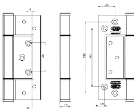
Screw hole fixing dimensions
