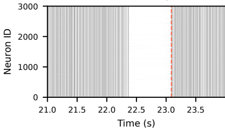
Neurons rasterplot
