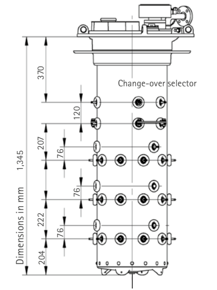
Installation length VVS® III 400 D
