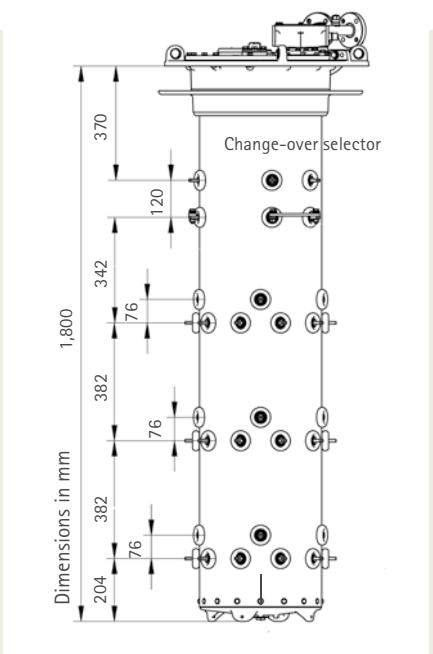
Installation length VVS® III 400 D
