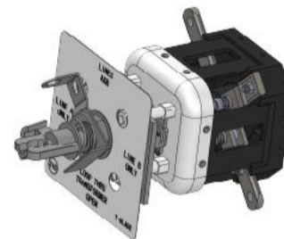
—15/25kV Single Phase Four-position Loadbreak Switch
