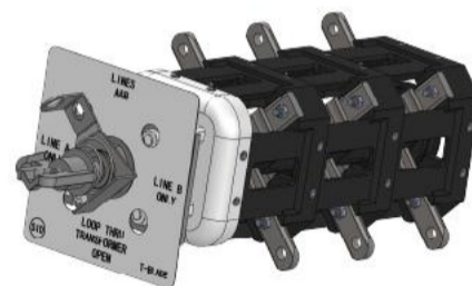
—15/25kV Three Phase Four-position Loadbreak Switch
