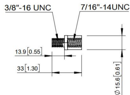
Removable nut
