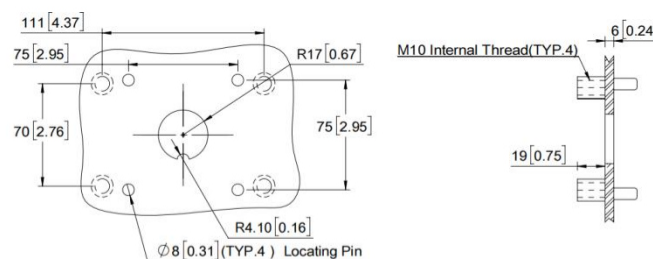
—Mounting hole & welding bolt
