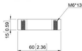
Mount Base(optional part)
