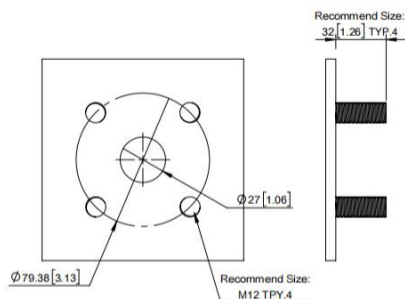
Fig 4 : Mounting Hole & Welding Bolt
