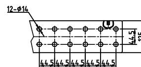
LV BUSHING
