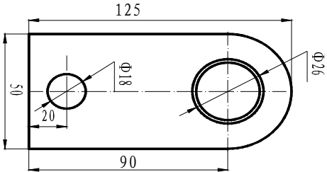
项4尺寸
