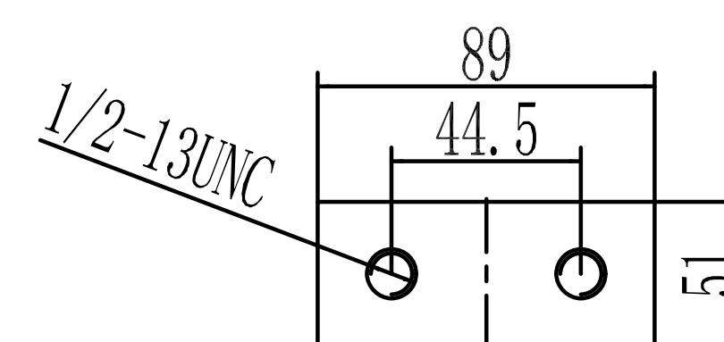
GROUND PAD STAINLESS STEEL
