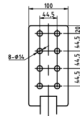
Lv bushing
