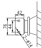
LV BUSHING TERMINAL DETAIL
