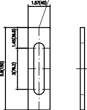
HOLD-DOWN PLATE DETAIL
