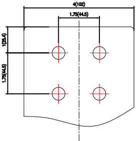
L.V. TERMINAL DETAIL
