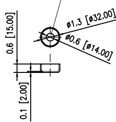
CUPPED WASHER DETAIL
