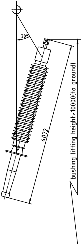
HV bushing height diagram
