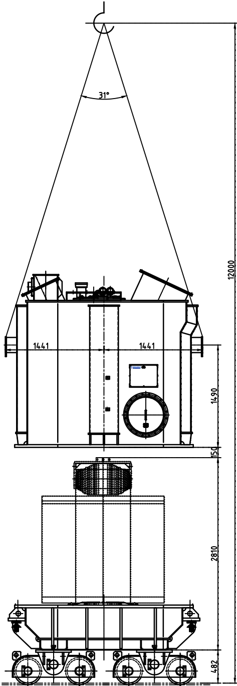
lifting height diagram
