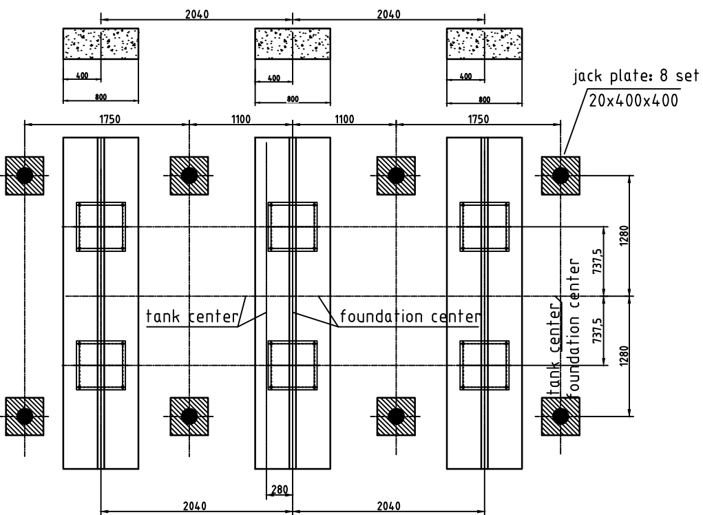
transformer foundation mounting diagram
