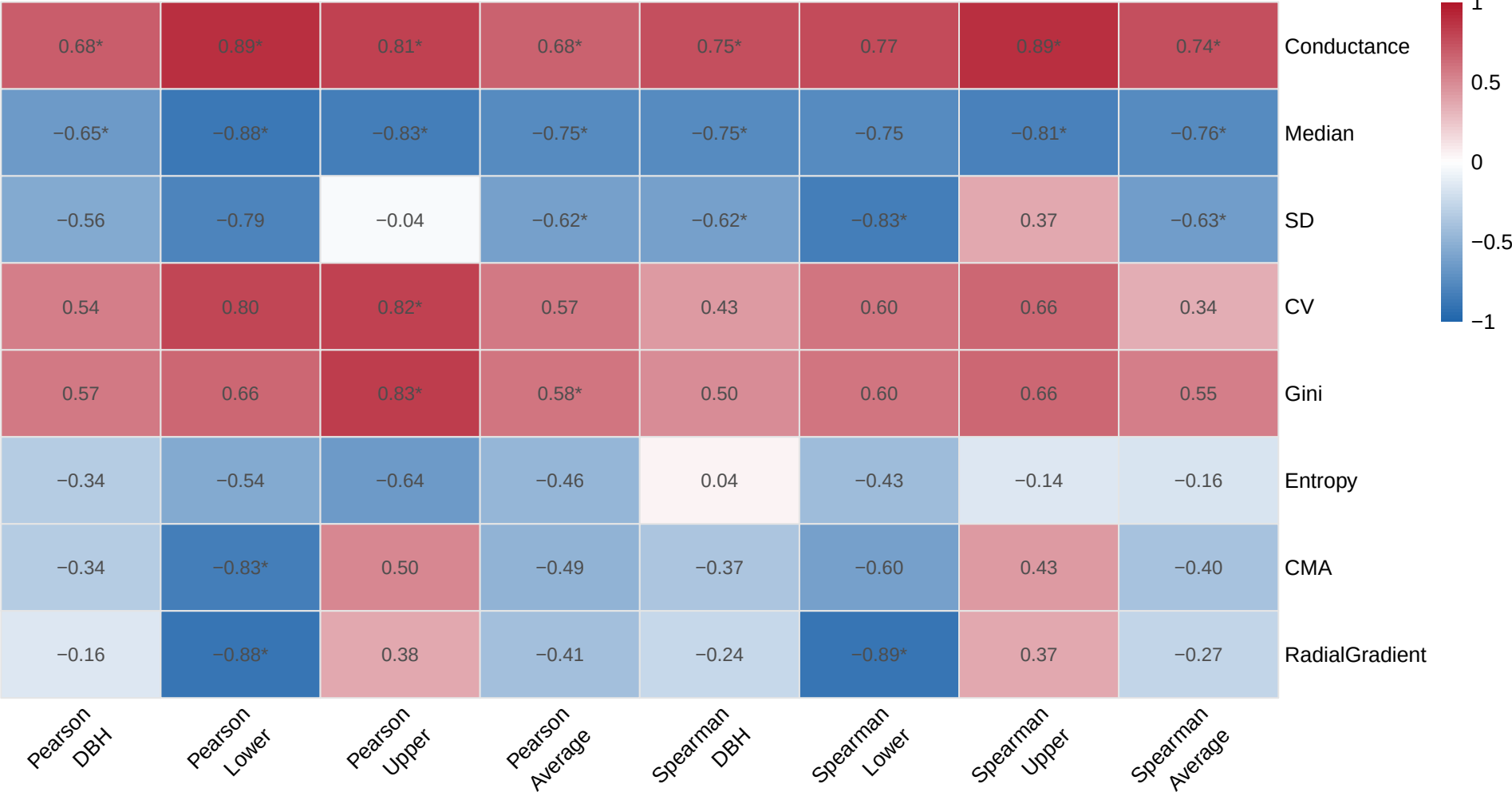
Correlations: ERT Metrics vs. Core Moisture (* p < 0.05)
