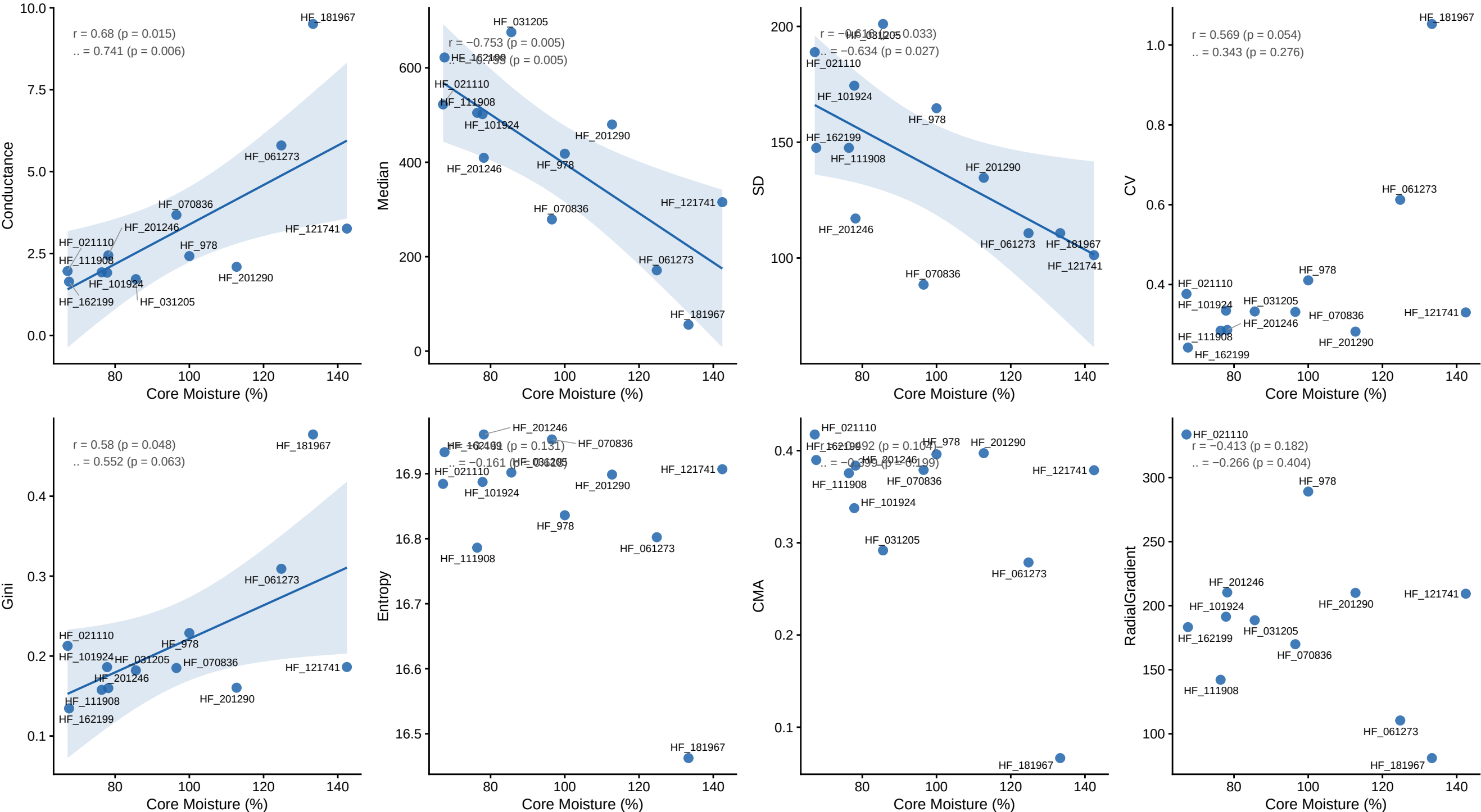
Average ERT Metrics (Across Heights) vs. Core Moisture
