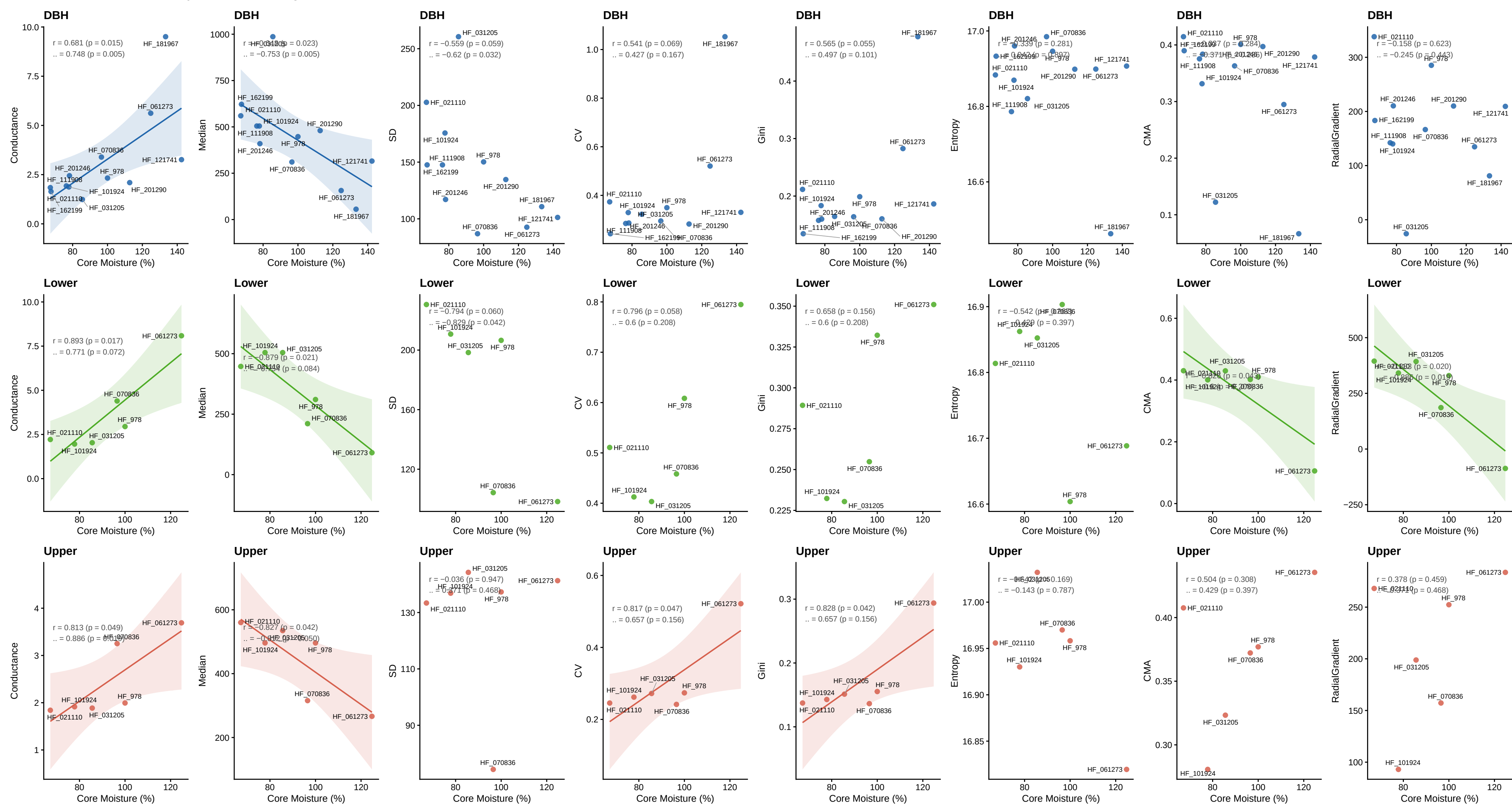
ERT Metrics vs. Core Moisture by Measurement Height
