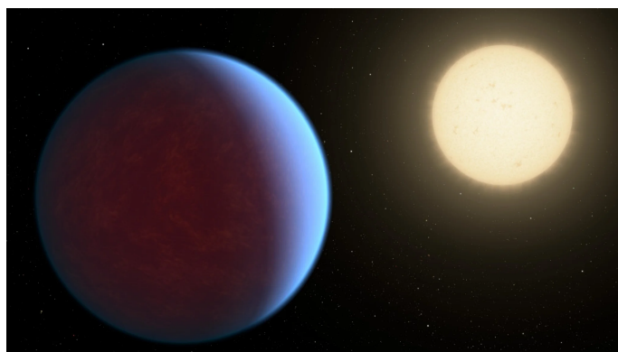
(b) creatioin of the light
