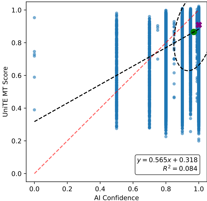
Calibration of Qwen3-1.7B thinking with monolithic prompt, aggregated on languages
