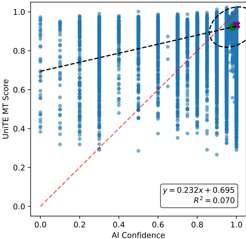
Calibration of Qwen3-14B thinking with iterative prompt, aggregated on languages
